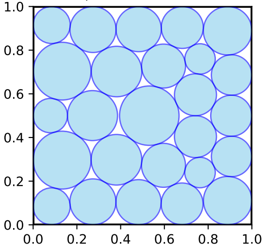
AlphaEvolve
