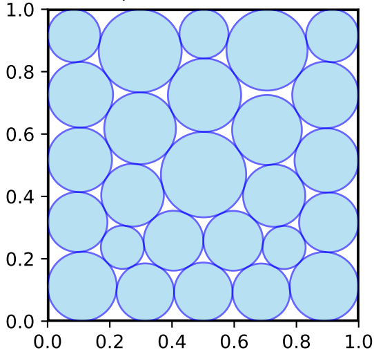
CodeEvolve
