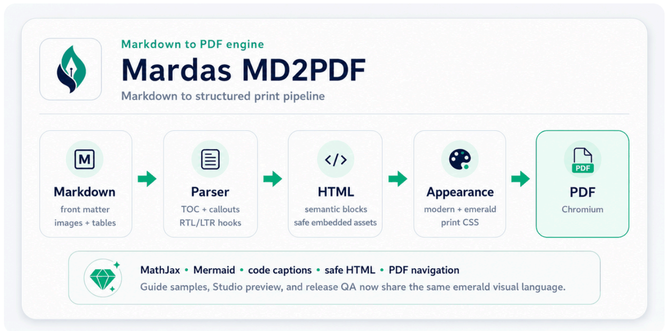
Figure 1. Architecture overview.
