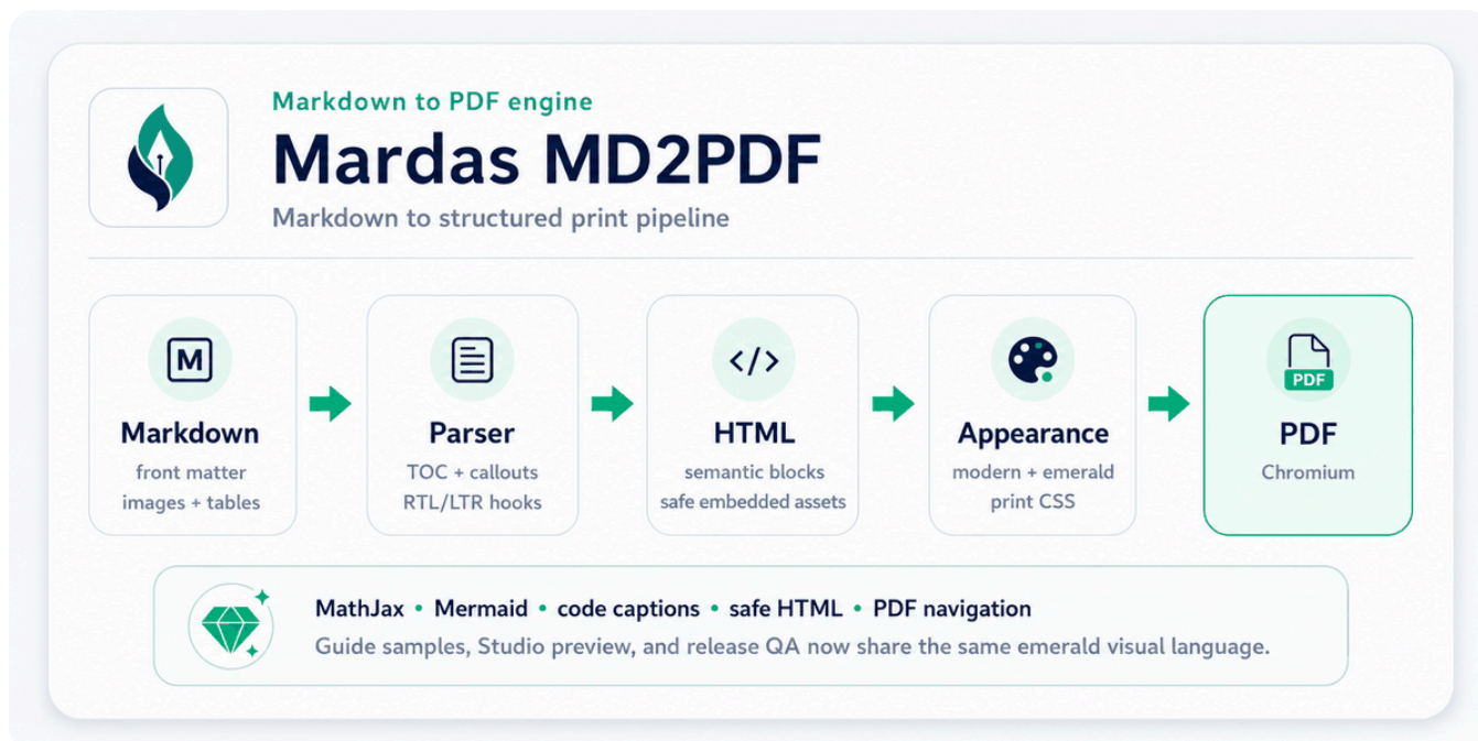
Figure 1. Architecture overview.
