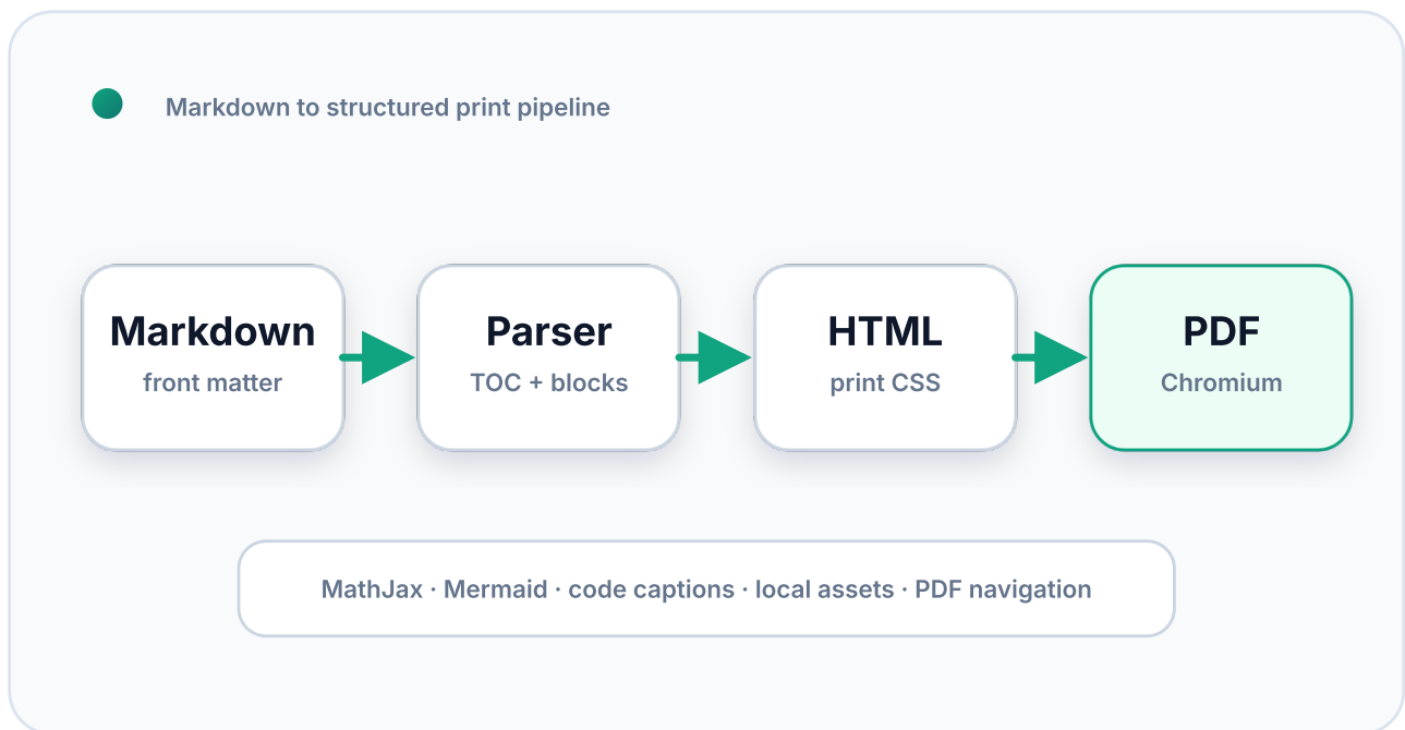
Figure 1. Architecture overview.
