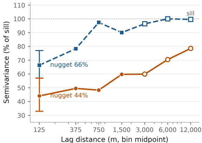
(b) Empirical semivariogram of \log_{10}(Q/s)
