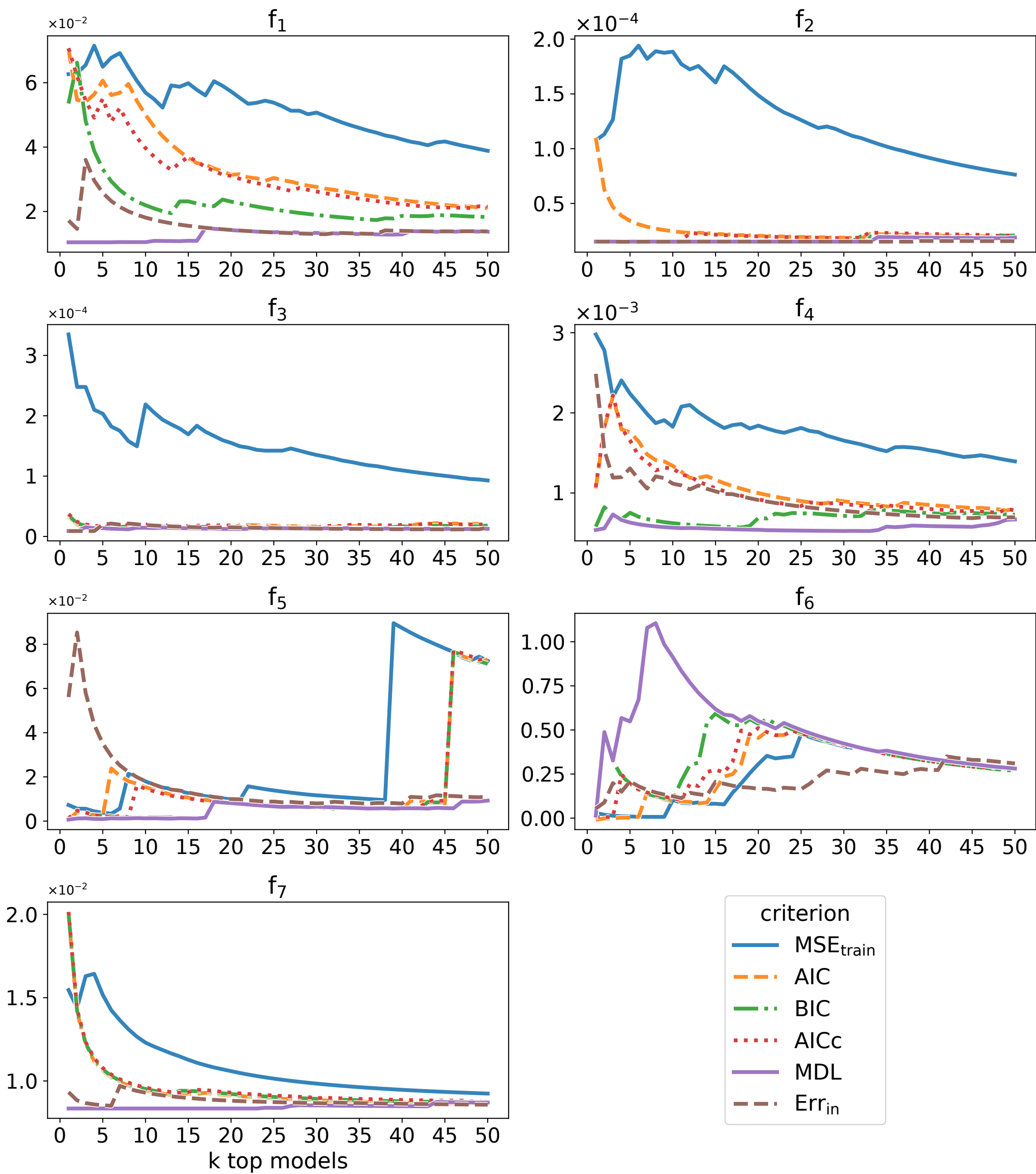
Average MSE test
