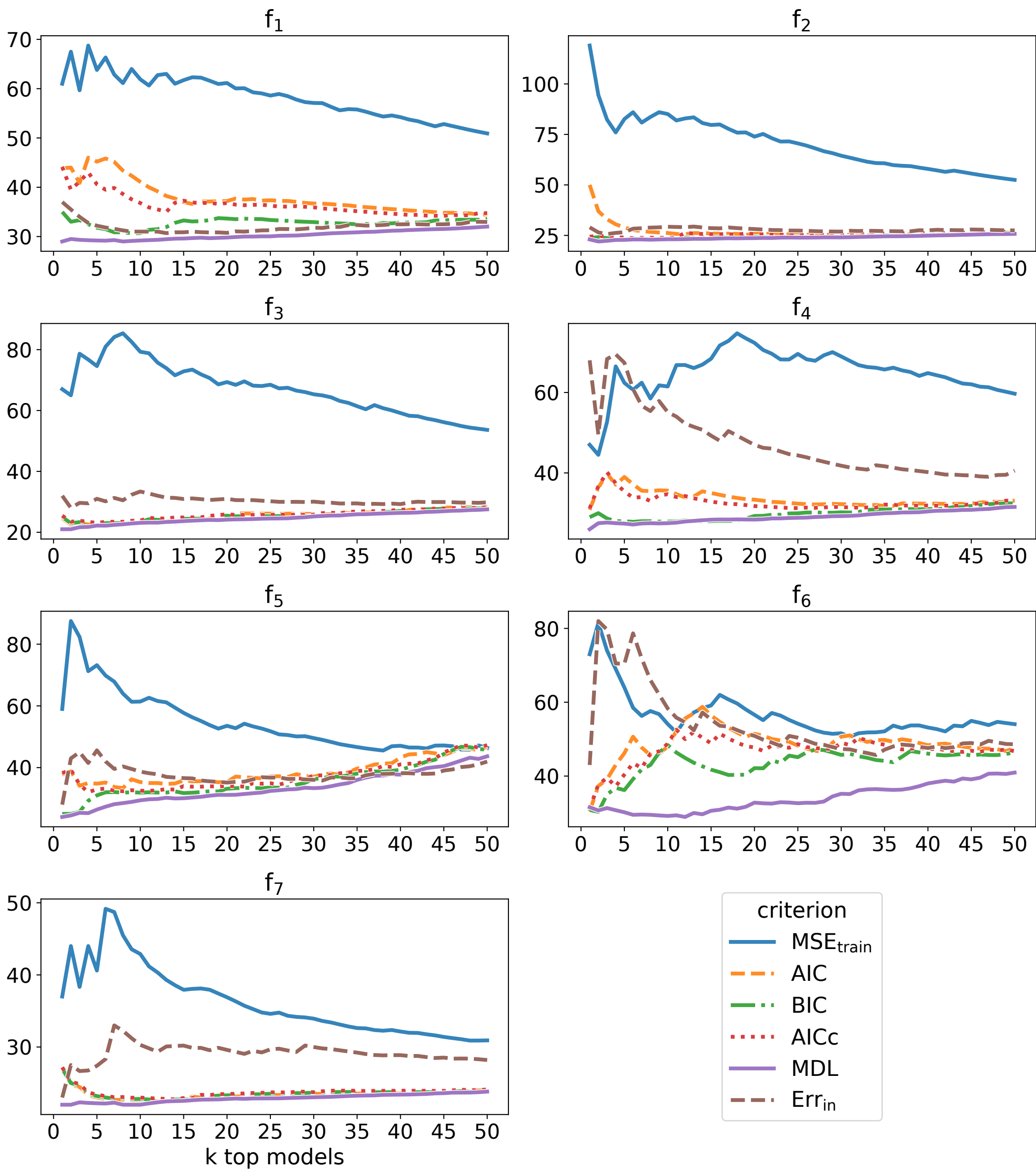
Average expression size
