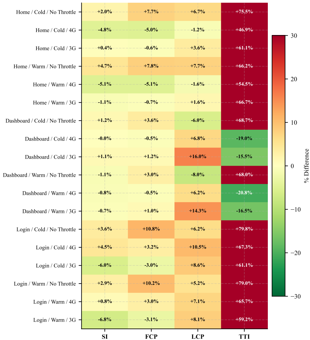
% Difference: MFE (Optimized) vs Monolith (Positive = MFE Slower)
