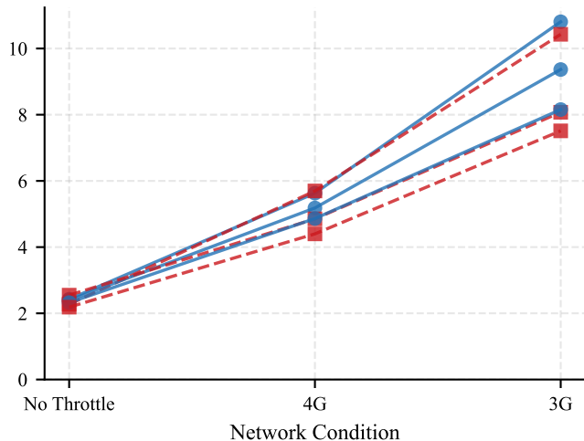
Largest Contentful Paint
