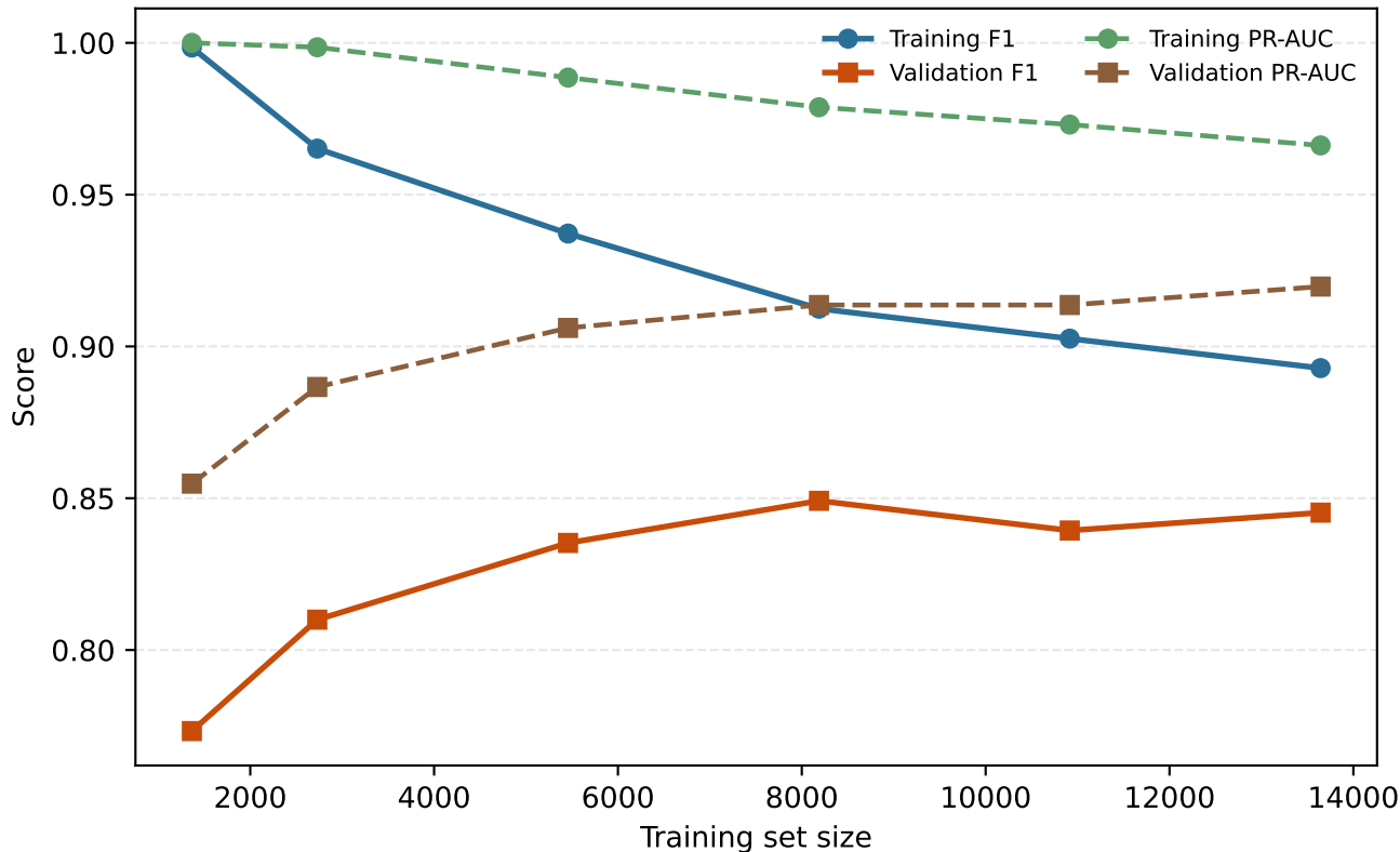
Learning curve for compact XGBoost model
