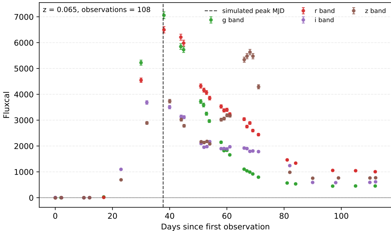
Example SPCC Type Ia light curve: SNID 319694
