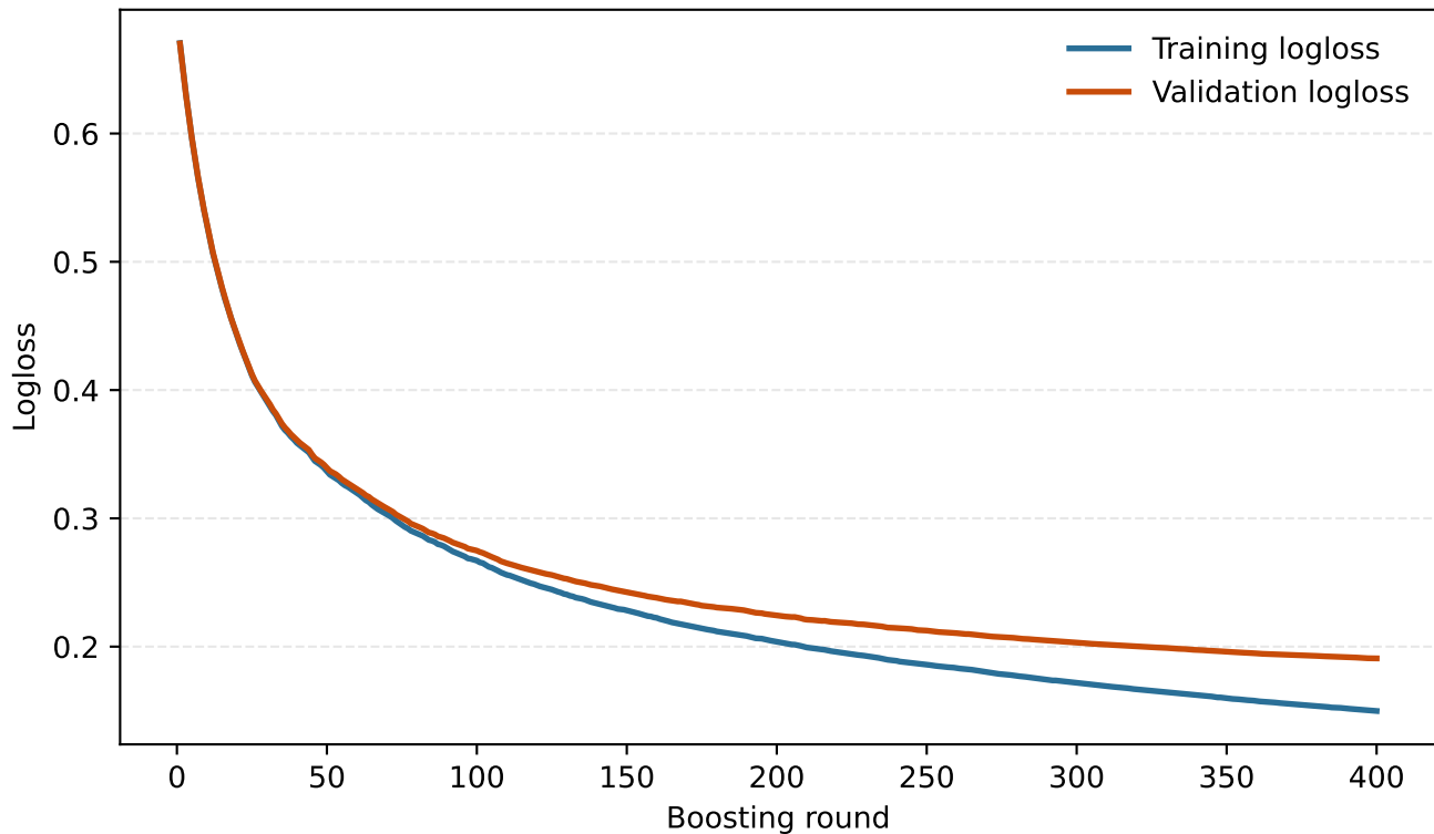
XGBoost convergence for compact feature model
