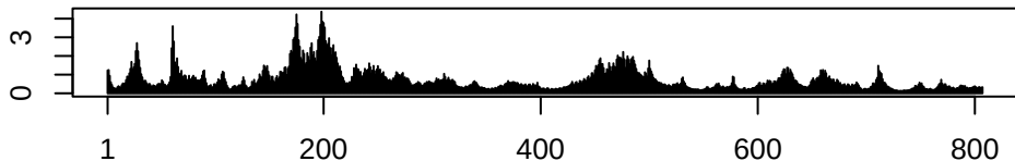
Fluctuations
