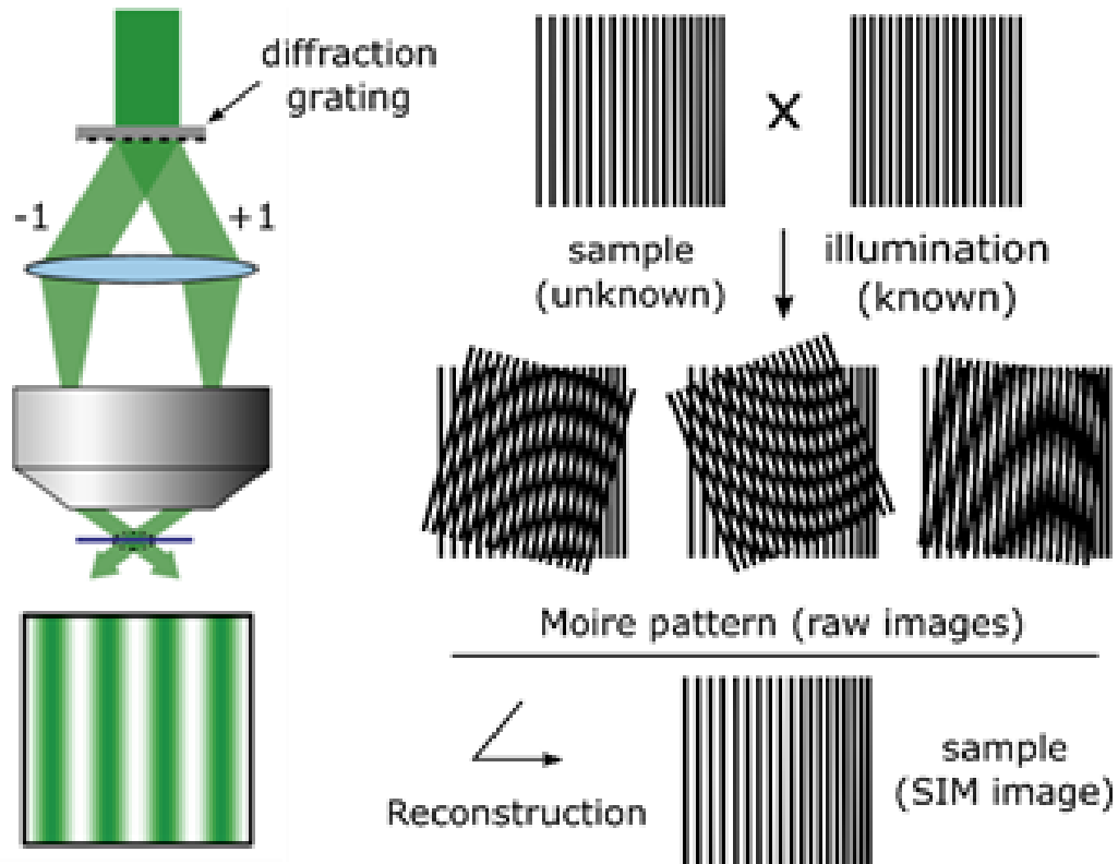
Abbildung 5.3: Structured Illumination Microscopy (Oxford Instruments 2025)
