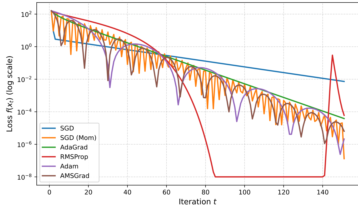
Quadratic Bowl Loss vs Iteration
