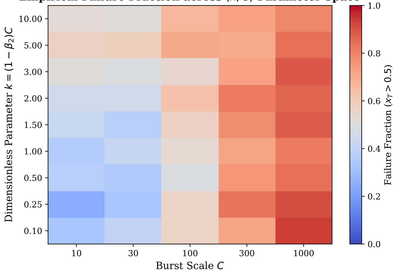
Empirical Failure Fraction across (k, C) Parameter Space
