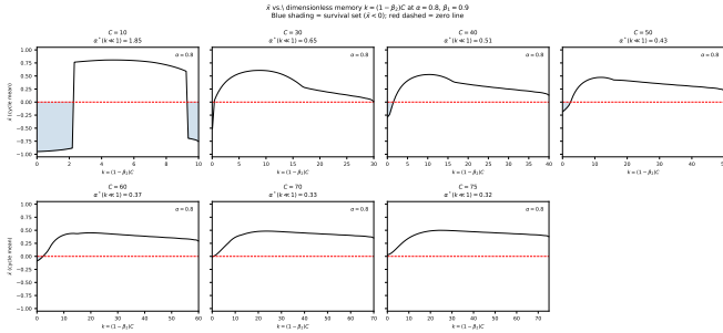
Figure 4: Cycle-averaged position \bar{x} vs. dimensionless memory k = (1 - \beta_2)C at \alpha = 0.8 , \beta_1 = 0.9 , T_{\text{cycles}} = 800 (source: results/mechanism_probes/xbar_vs_k_profiles.csv ). Blue shading marks the survival set ( \bar{x} < 0 ). The k -axis runs from 0 (large \beta_2 \rightarrow 1 , Regime II) to C (small \beta_2 \rightarrow 0 ). Red dashed: \bar{x} = 0 .
