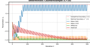
(a) Trajectory x_t over 500 steps.
