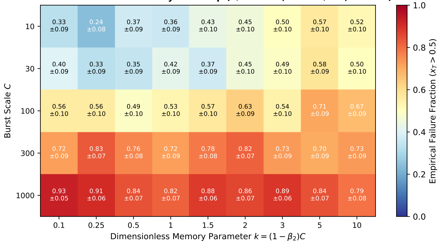
Stochastic Failure Probability Heatmap (4,500 runs, N = 100/\text{cell} , \delta = 0.10 )
