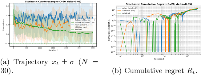
Figure 2: Stochastic counterexample replication ( C = 20, \delta = 0.05 ). Under constant step size \alpha = 0.8 , ADAM exhibits net positive drift and linear regret \Omega(T) , while AMSGRAD and ADAGRAD maintain negative mean trajectories towards the optimal basin.
