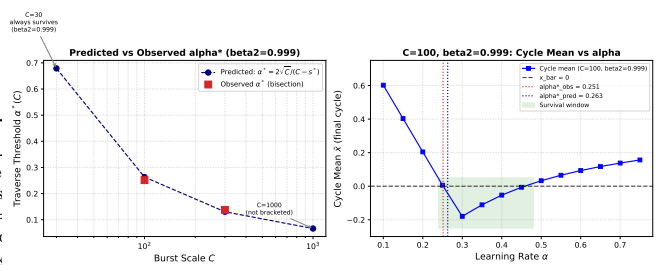
Figure 3: \alpha^* traverse threshold validation ( \beta_2 = 0.999 ). Predicted \alpha^*(C) = 2\sqrt{C}/(C - s^*) (filled circles, dashed), with s^* = \tau_1 \ln((1-\beta_1)C + 1) and \tau_1 = 1/(1-\beta_1) . The second panel shows the cycle mean \bar{x} vs. \alpha at C = 100 : the sign change from positive (failure) to negative (survival) and back confirms a survival window, with the lower crossing matching the predicted \alpha^* = 0.263 to within 5%.
