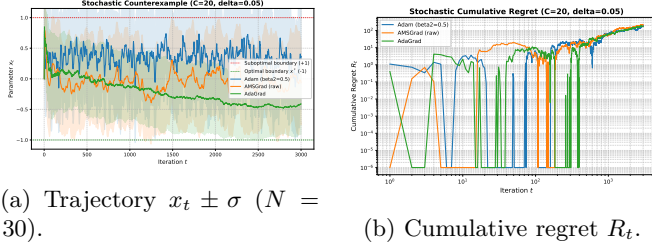
Figure 2: Stochastic counterexample replication ( C = 20, \delta = 0.05 ). ADAM exhibits net positive drift and linear regret \Omega(T) , while AMSGRAD and ADAGRAD enforce sublinear regret.
