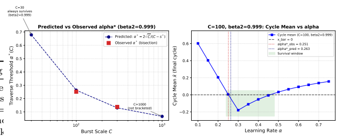
Figure 3: \alpha^* traverse threshold validation ( \beta_2 = 0.999 ). Predicted \alpha^*(C) = 2\sqrt{C}/(C - s^*) (filled circles, dashed), with s^* = \tau_1 \ln((1 - \beta_1)C + 1) and \tau_1 = 1/(1 - \beta_1) . The second panel shows the cycle mean \bar{x} vs. \alpha at C = 100 : the sign change from positive (failure) to negative (survival) and back confirms a survival window, with the lower crossing matching the predicted \alpha^* = 0.263 to within 5%.
