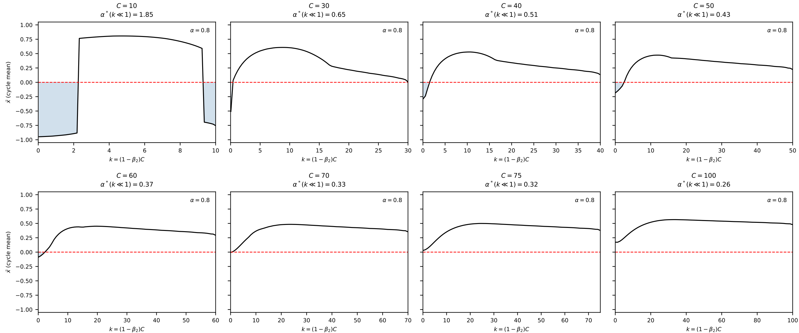
\bar{x} vs. \ dimensionless memory k = (1 - \beta_2)C at \alpha = 0.8 , \beta_1 = 0.9 Blue shading = survival set ( \bar{x} < 0 ); red dashed = zero line
