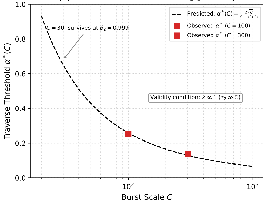
(a) Predicted vs. Observed \alpha^* ( \beta_2 = 0.999 )
