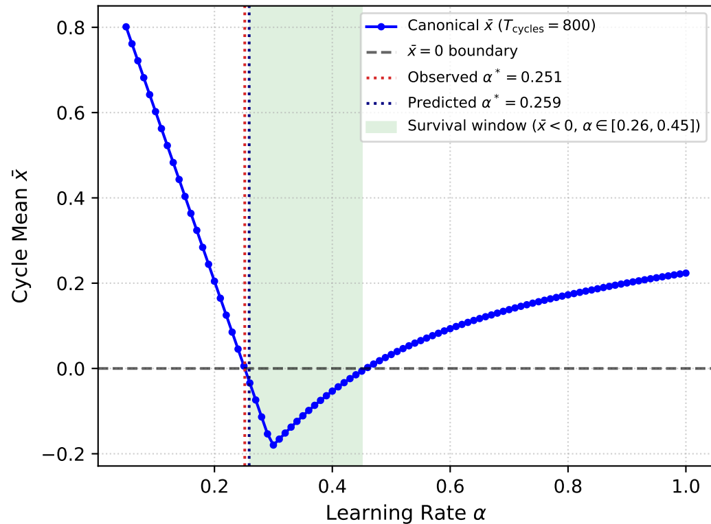
(b) C = 100, \beta_2 = 0.999 : Cycle Mean vs. \alpha
