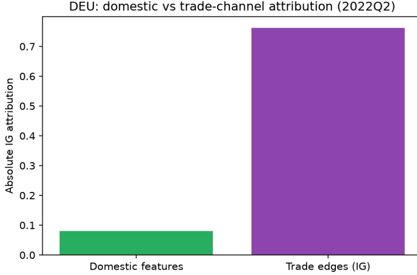
Figure 2: Decomposition of Integrated Gradients attributions for Germany during the 2022 energy shock (2022Q2).
