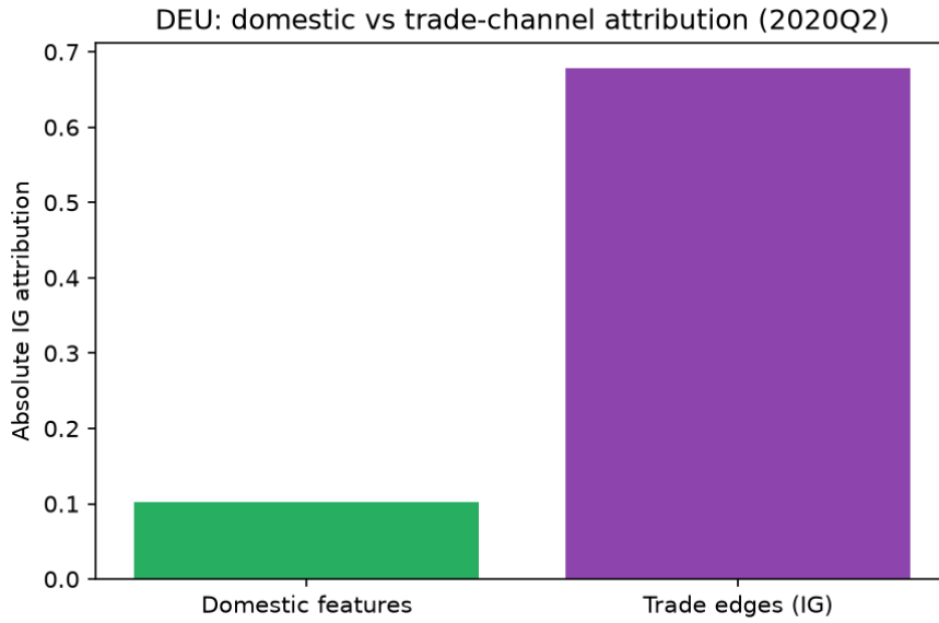
Figure 1: Decomposition of Integrated Gradients attributions for Germany during the COVID supply-chain period (2020Q2).
