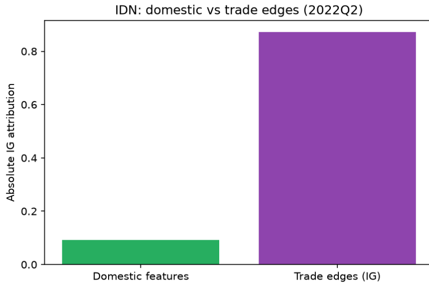
Figure 4: Indonesia trade-versus-domestic attribution ratio (9.44), highest in the panel at 2022Q2.
