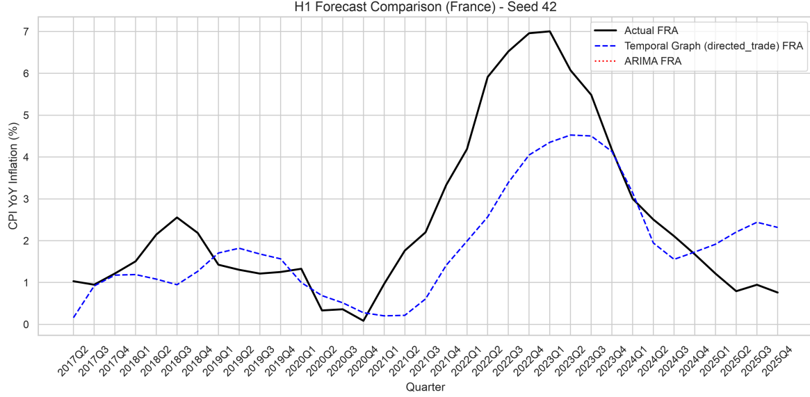
Figure 2: Figure 2: Forecast comparison (France, Seed 42, H=1 ). Comparison of Temporal Graph (directed_trade variant) and ARIMA forecasts against actual CPI YoY inflation. The plot illustrates where the neural model deviates from classical baselines during inflation transition periods.
