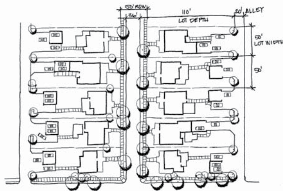
TYPICAL NEIGHBORHOOD LAYOUT
