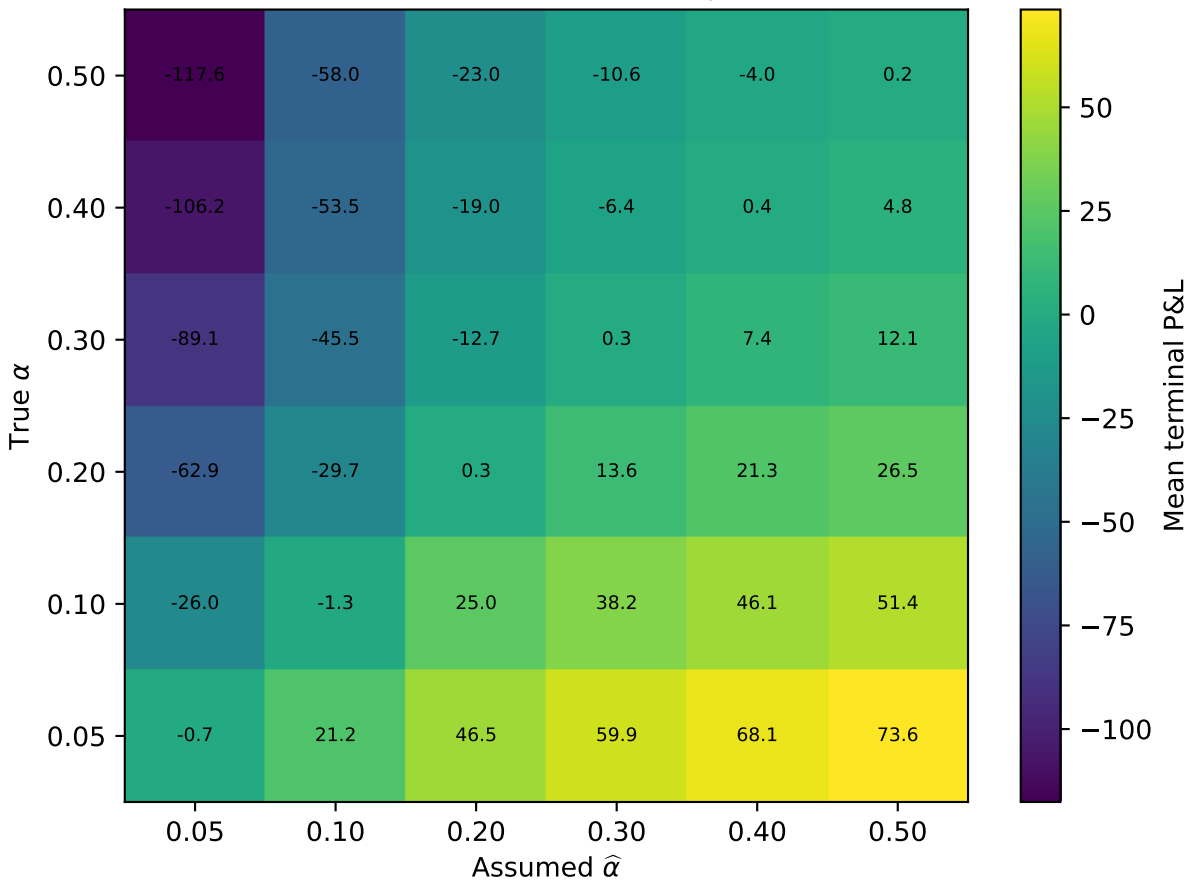
Terminal P&L under model misspecification
