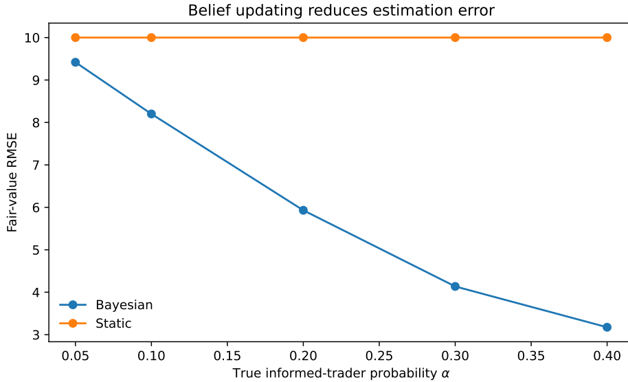
Figure 3: Fair-value RMSE under static and Bayesian strategies.
