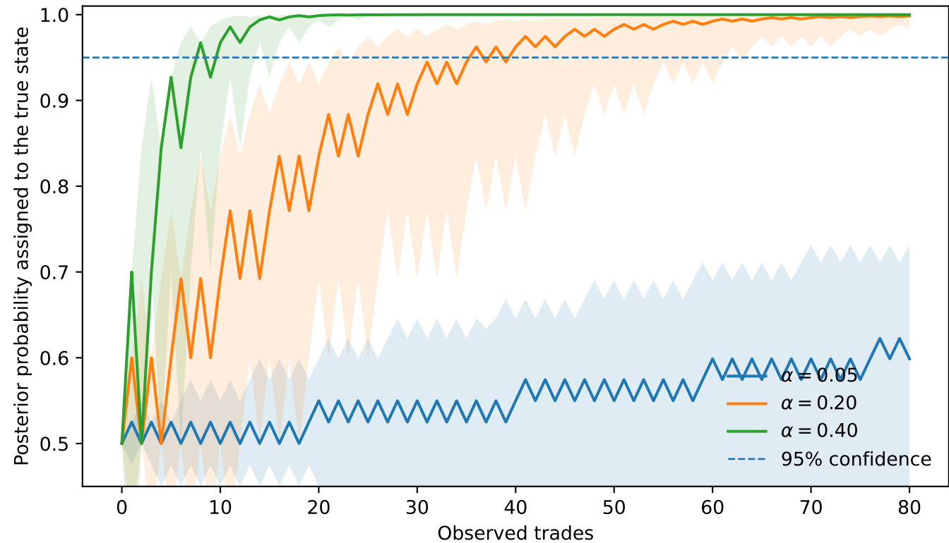
Price discovery from order direction
