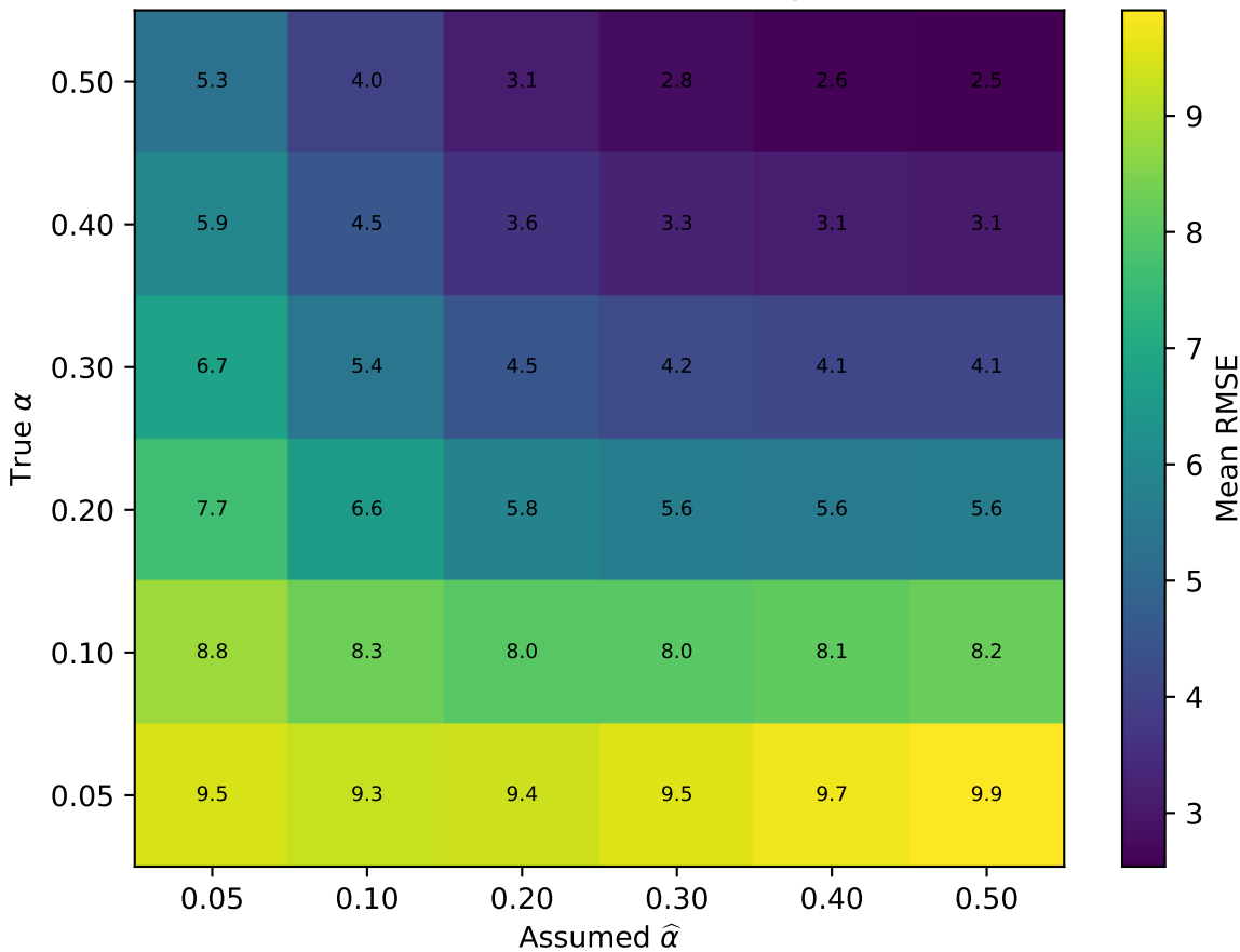
Fair-value error under model misspecification
