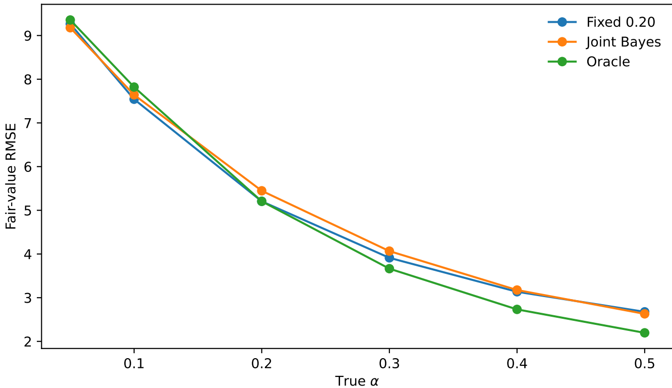
Known, fixed, and jointly inferred information intensity
