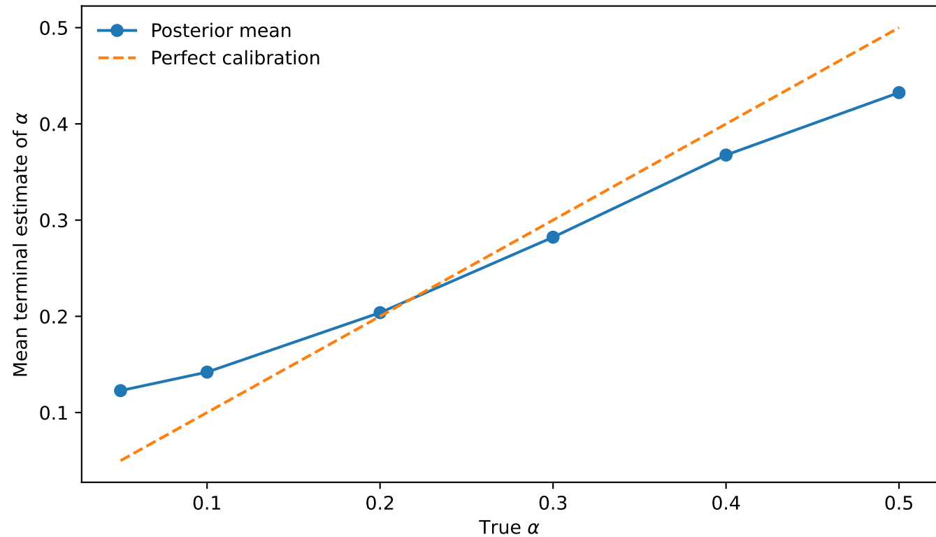
Calibration of the joint Bayesian filter
