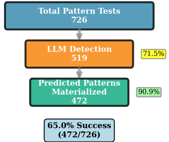
Fig. 7. Pattern detection validation funnel showing progression from 726 total tests to 519 detections (71.5% detection rate) to 472 materialized predictions (90.9% accuracy), yielding 65.0% overall success rate.
