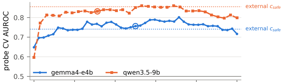
(a) hidden-state probe, layer by layer (open circle = median layer, used for the verdict)
