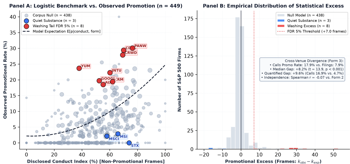
Figure 17: Empirical Identification of AI Washing: Panel A tests conditional promotional excess via frame-level logistic regression on conduct and form mix (identifying 8 firms in the washing tail at 5% FDR). Panel B displays the distribution of promotional excess ( k_{obs} - k_{exp} ) and cross-venue divergence metrics.
