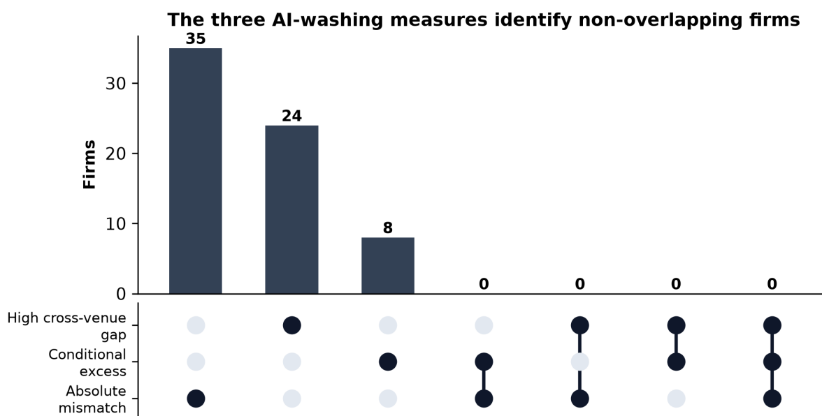
Figure 18: The three AI-washing measures flag different firms: set sizes and overlaps (UpSet-style plot). Absolute mismatch = 35 firms in the top promotional tercile with zero grounded (deployed, named-product) activity; conditional excess = 8 firms flagged by the binomial test; high cross-venue gap = 24 firms one SD or more above the mean call-minus-filing promotional gap.
