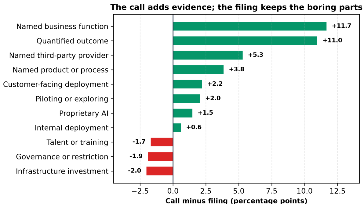
Figure 13: Same activity, different evidence: call-minus-filing gap in how often each activity carries a given piece of evidence, ordered from largest to smallest (percentage points).
