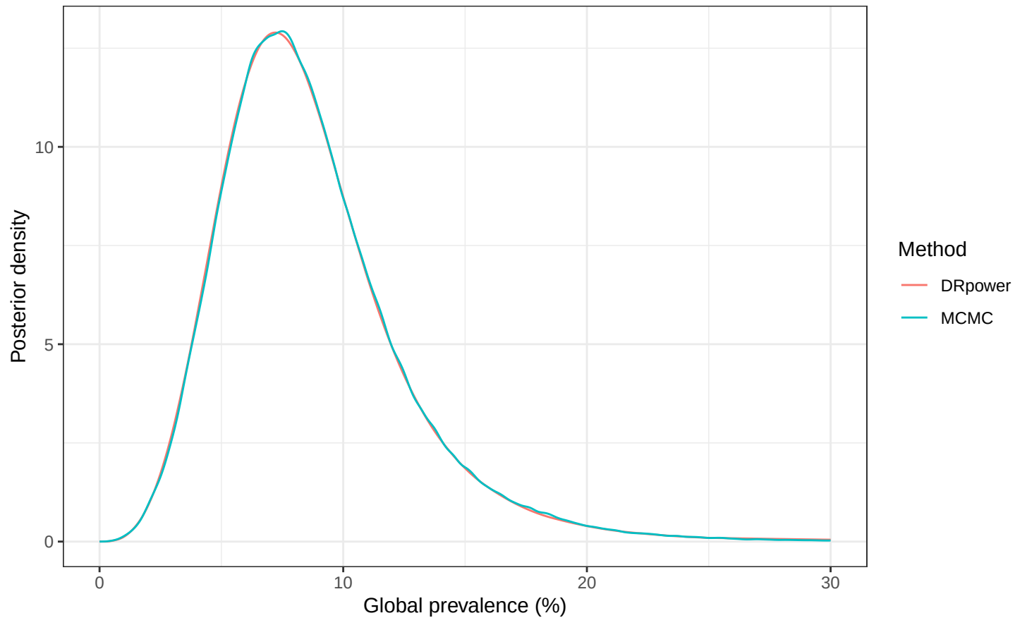
Comparison of DRpower vs. MCMC posterior distributions
