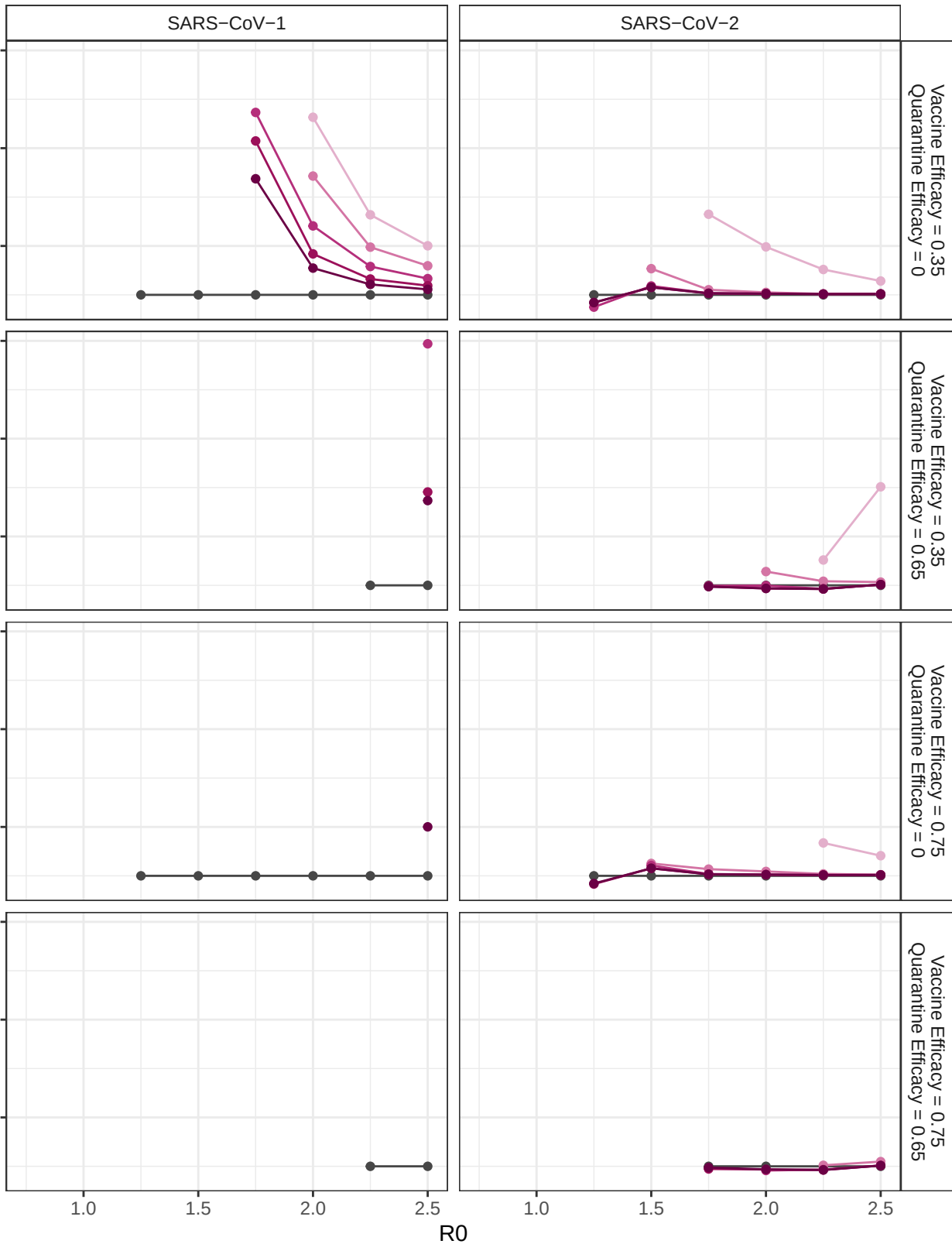
Fold Increase in Time to Epidemic Threshold
