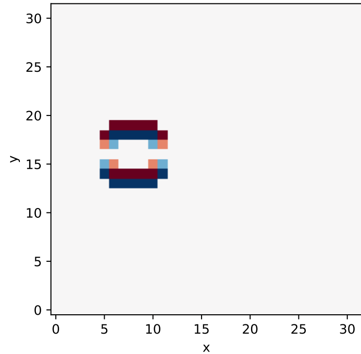
Persistence
