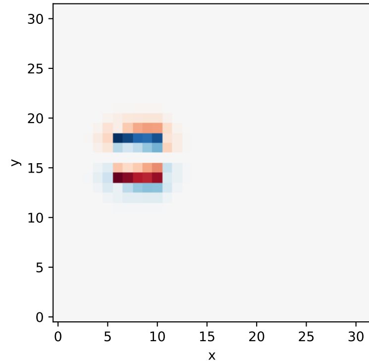
RK4 (dt=0.001)
