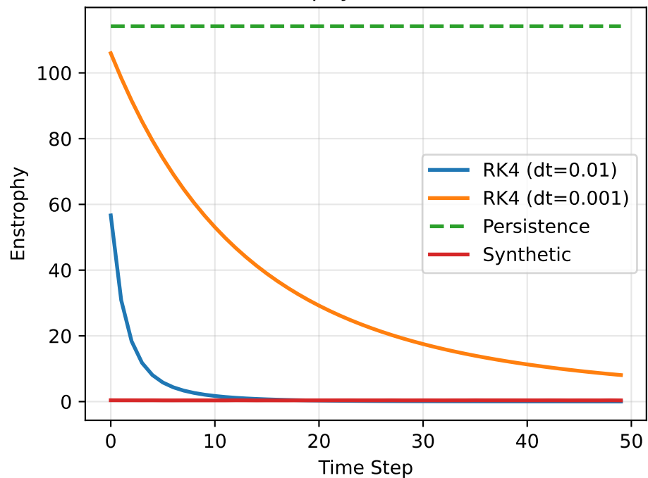
Enstrophy Time Series
