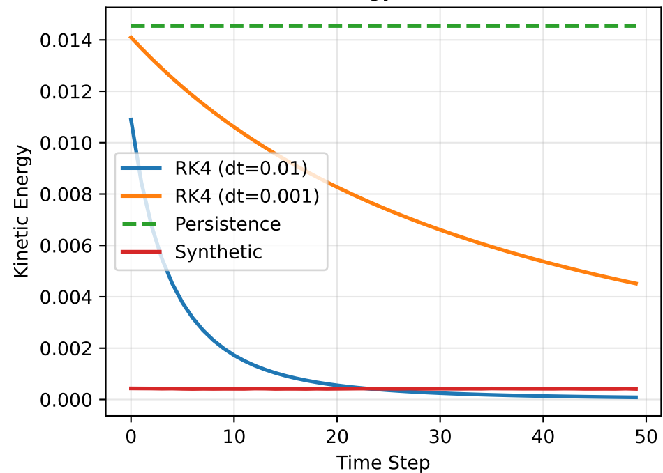
Kinetic Energy Time Series
