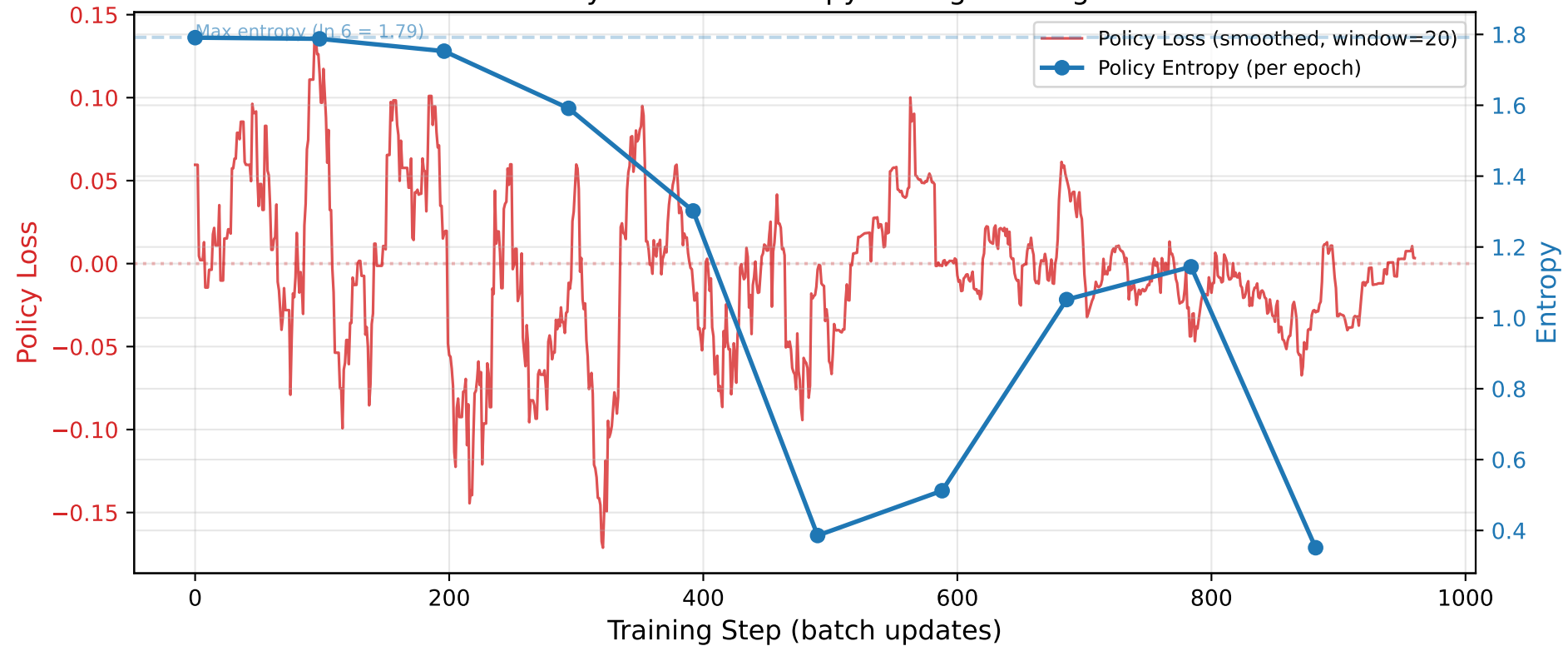
Policy Loss and Entropy During Training
