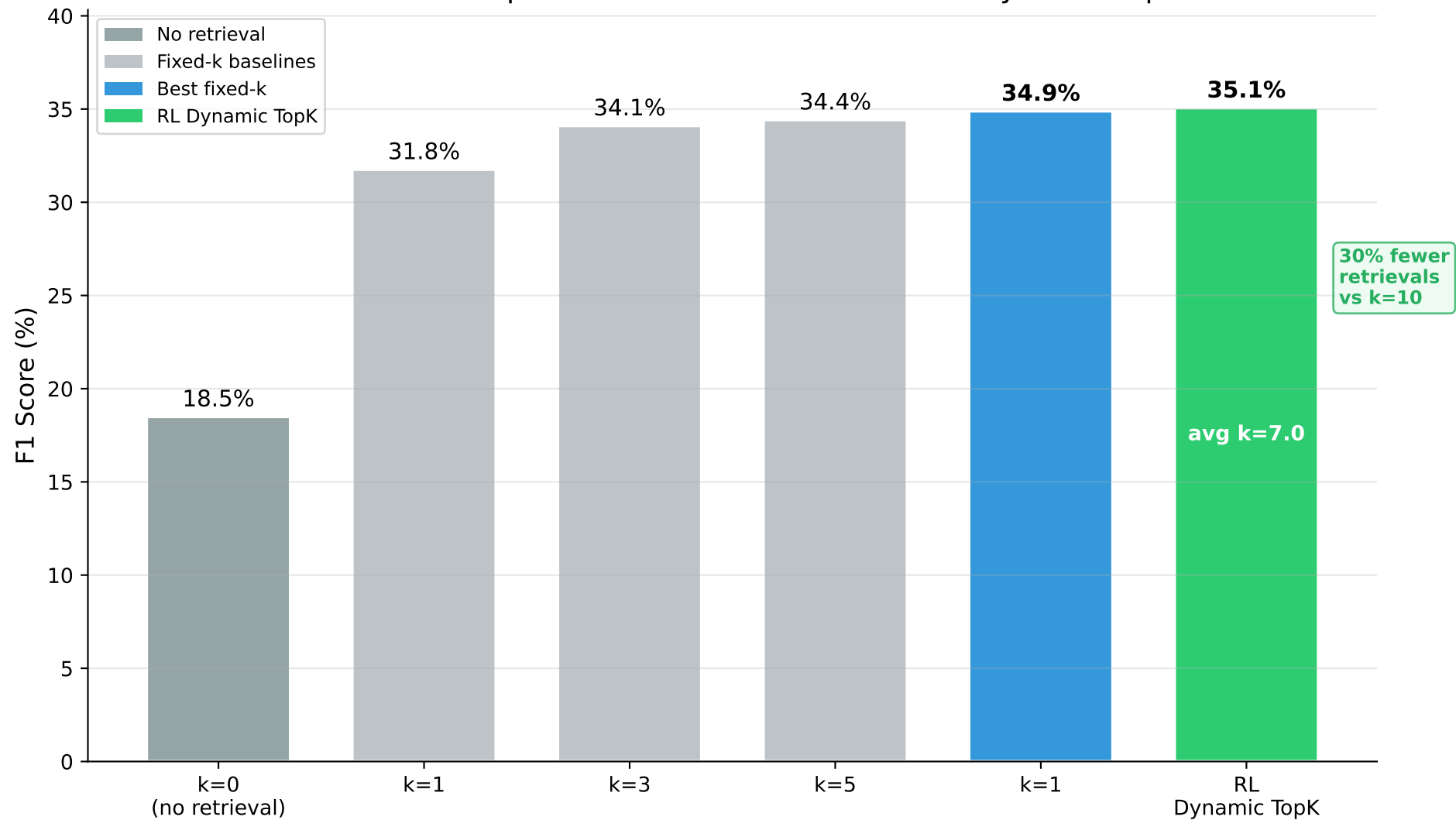
Controlled Comparison: Fixed-k Baselines vs RL Dynamic TopK
