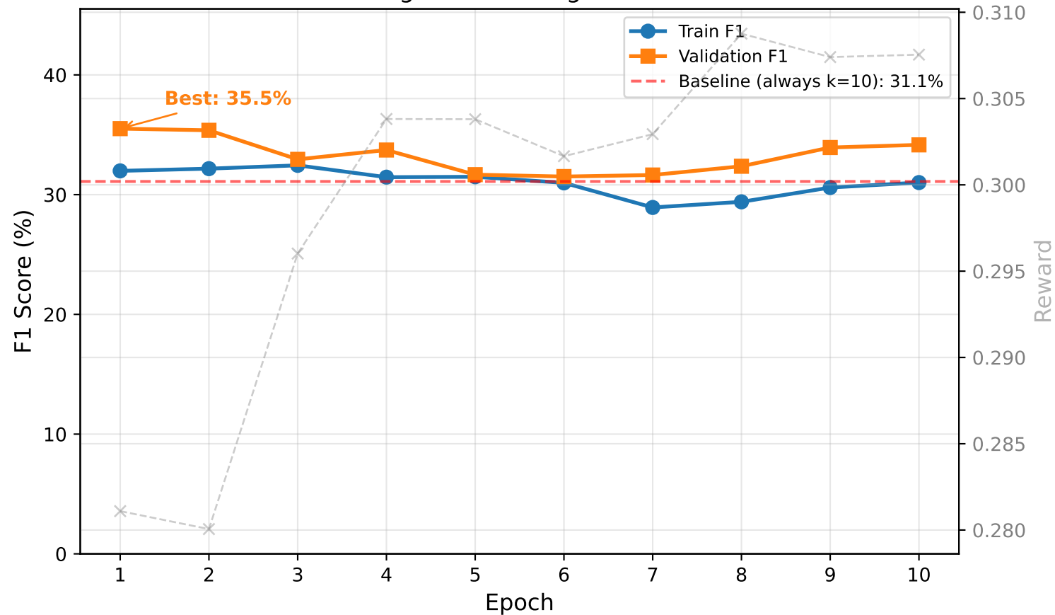
F1 Learning Curve: RL Agent vs Baseline
