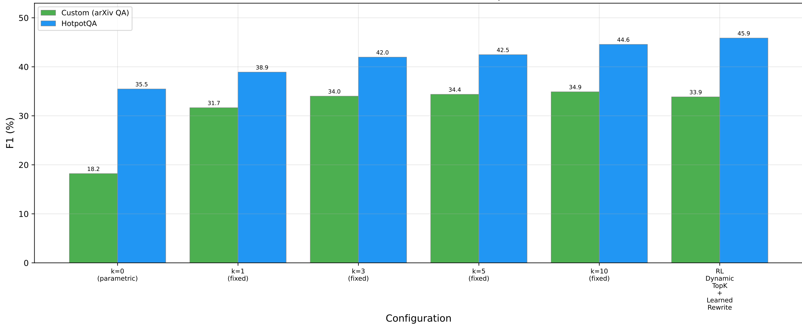
Cross-Dataset RAG Performance Comparison
