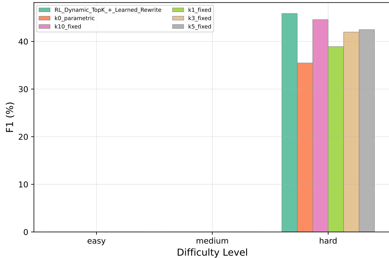
F1 by HotpotQA Difficulty Level
