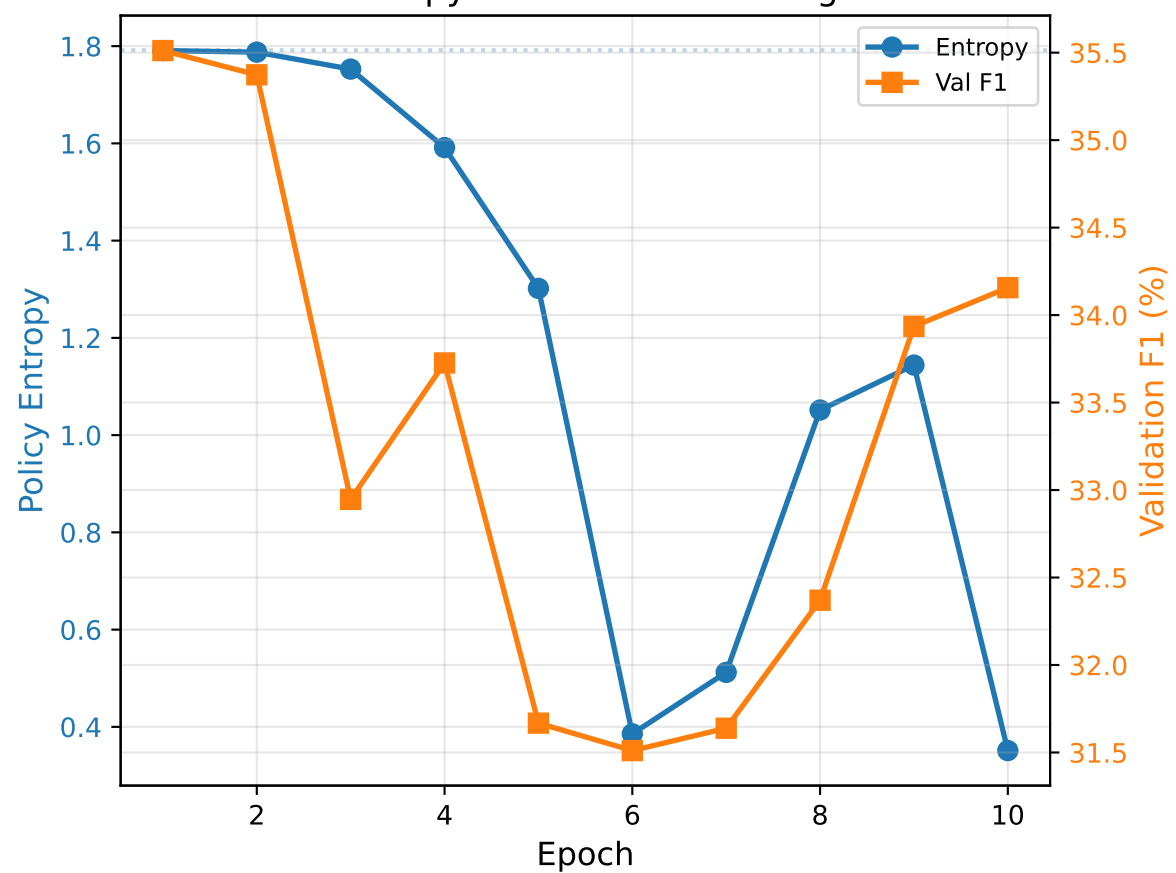
Entropy and F1 Over Training
