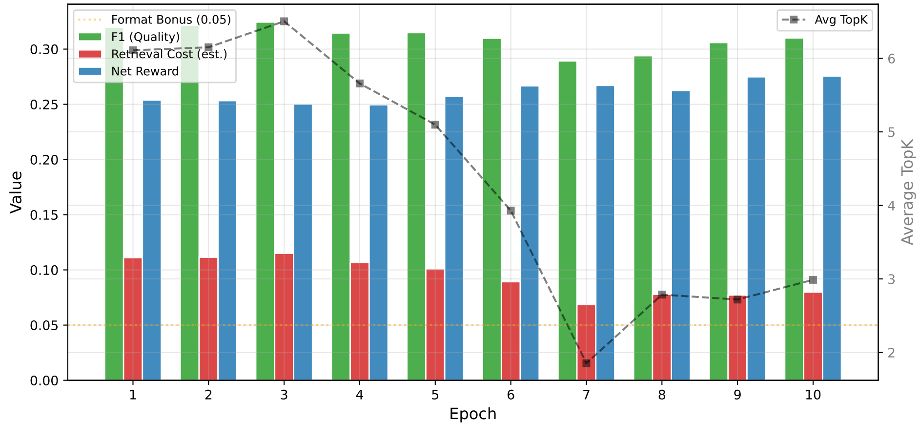
Reward Decomposition Across Training
