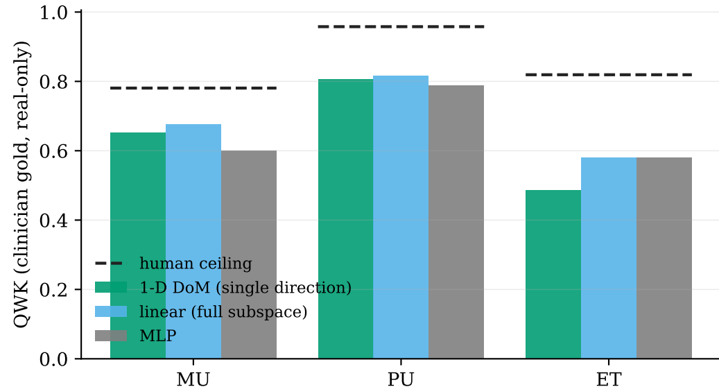
Probe head: does ET need more than one direction?
