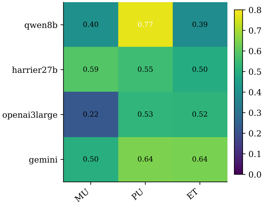
Golden QWK by embedder × axis
