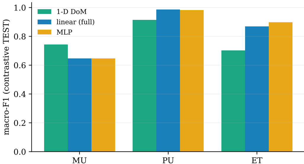
Linear sufficiency
