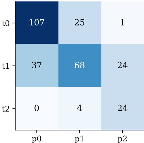
MU golden (real) confusion
