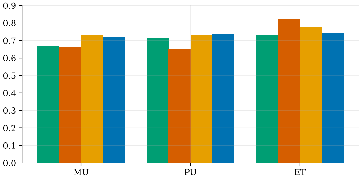
real-only macro-F1
