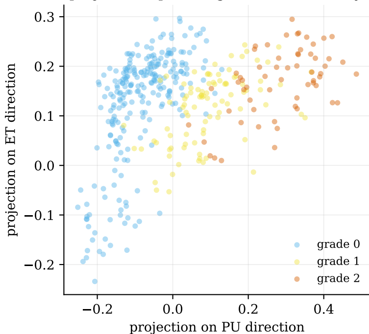
PU vs ET projection (qwen8b/generic), colored by PU grade
