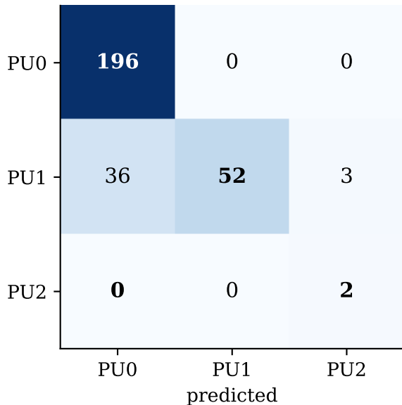
gpt-oss-120b
