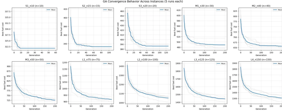
Figure 3: Convergence curves for all ten instances. Grey: individual runs; blue: mean of the five runs.
