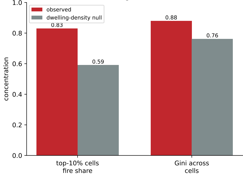
Observed vs null (fire-weighted mean over 4964 LSOAs)
