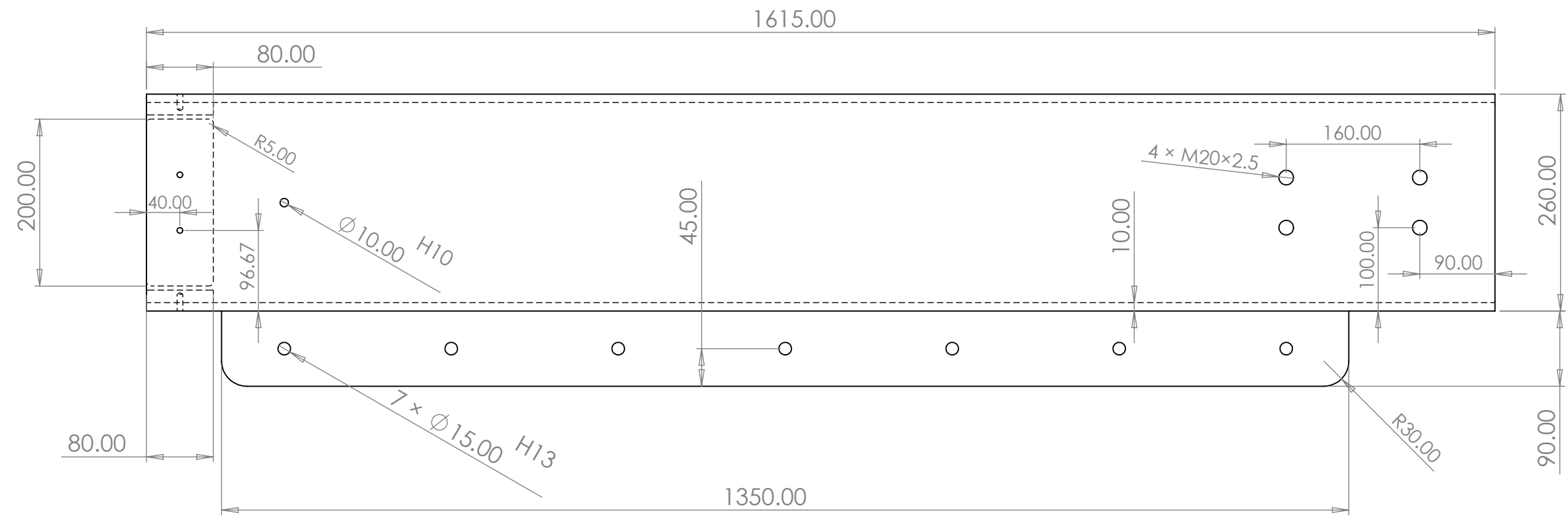
Front View
