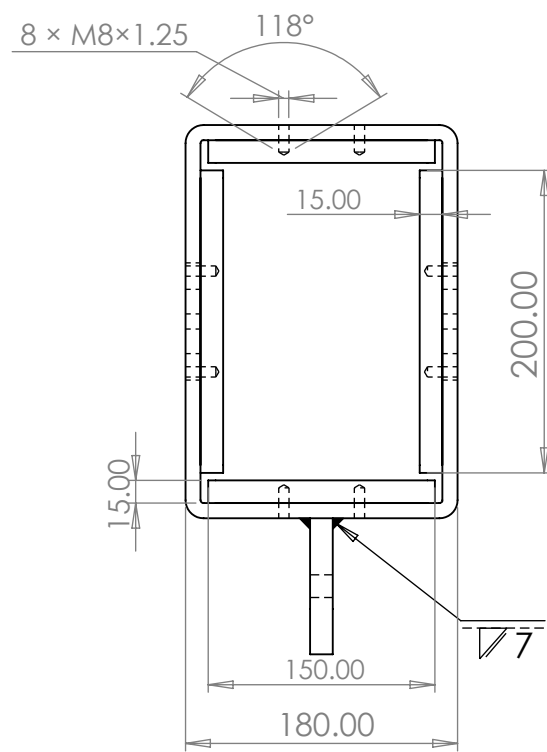
Left View
